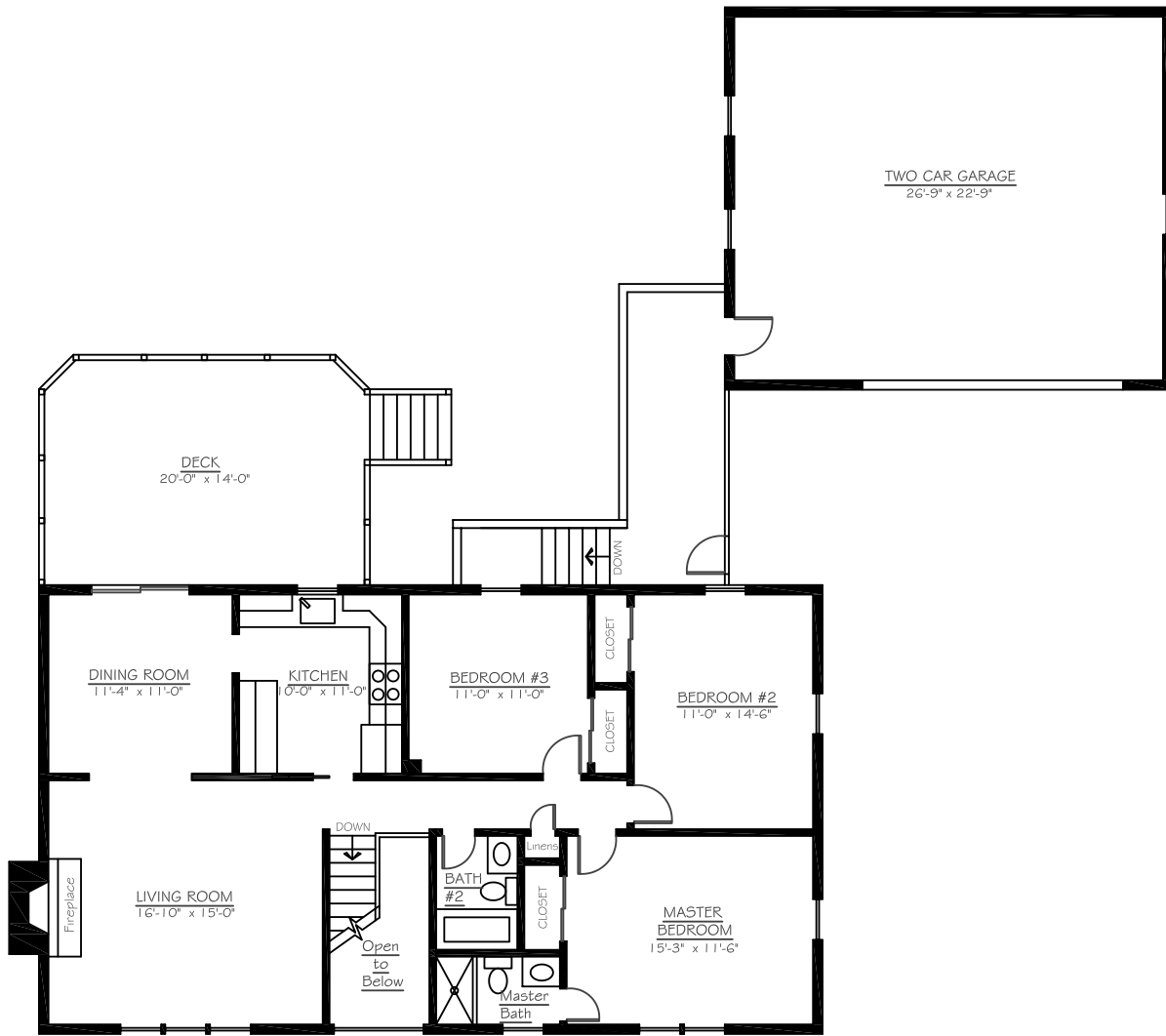
MAIN LEVEL
